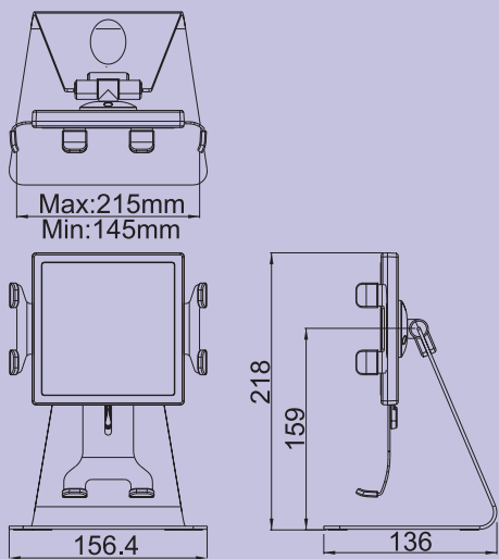
Physical Dimensions (mm) Multimedia Devices Such as iPad Kindle DX ViewPad,Eee Pad
